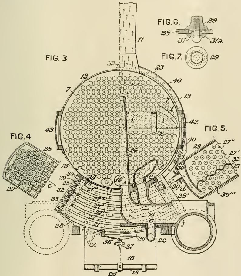
FORNEY'S FEED-WATER HEATER—TRANSVERSE SECTION
